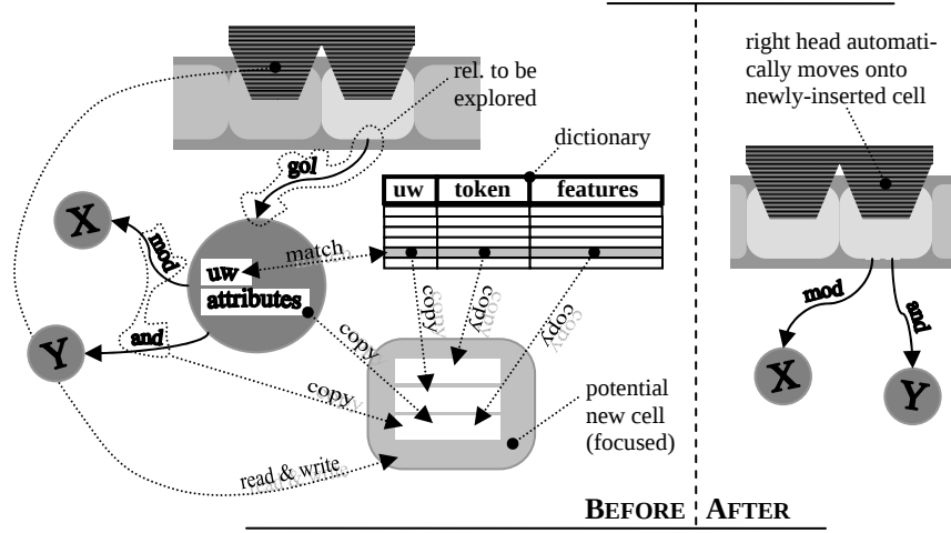
Fig. 2. Before and after node transference
